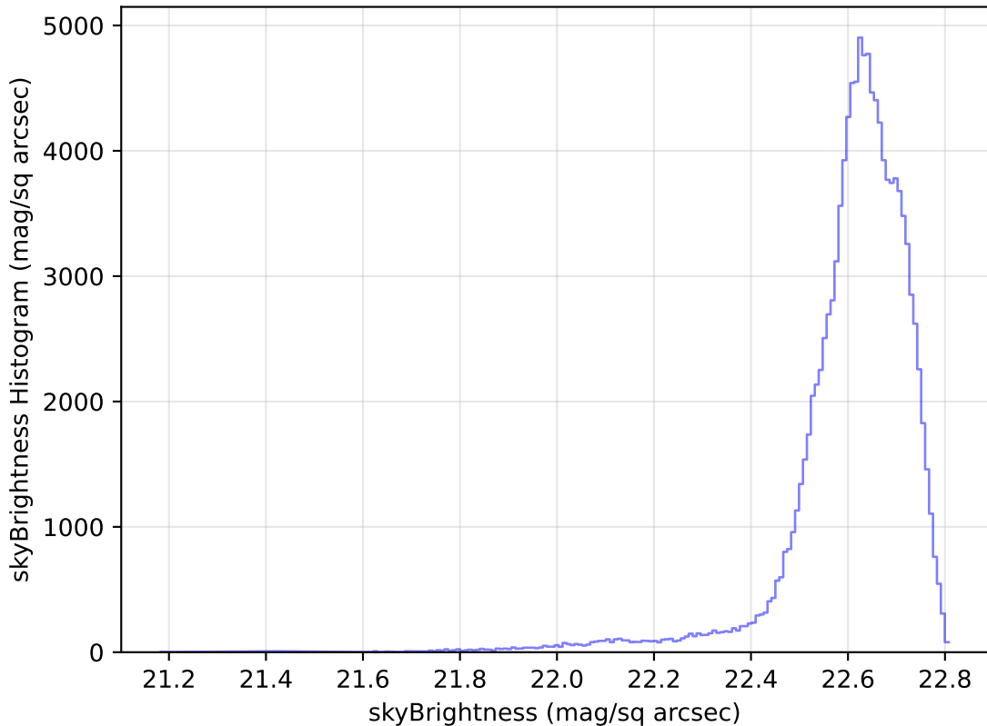
too_elab_r64_d2_giz_v3.4_10yrs WFD u band: skyBrightness Histogram
