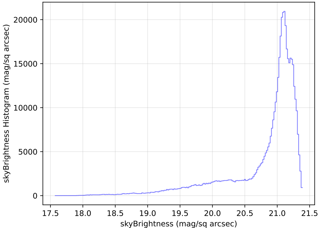
too_elab_r64_d2_giz_v3.4_10yrs WFD r band: skyBrightness Histogram
