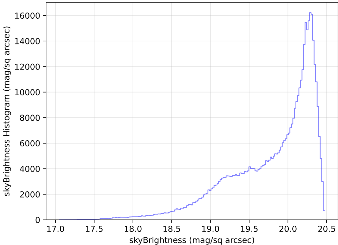
too_elab_r64_d2_giz_v3.4_10yrs WFD i band: skyBrightness Histogram
