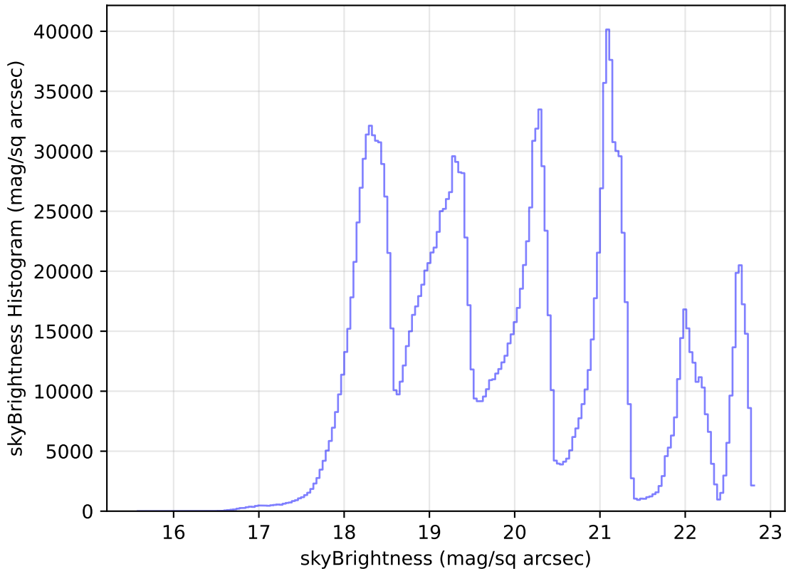
too_elab_r64_d2_giz_v3.4_10yrs WFD all bands: skyBrightness Histogram
