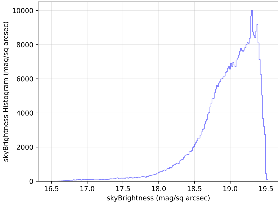
too_elab_r64_d2_giz_v3.4_10yrs All sky z band: skyBrightness Histogram
