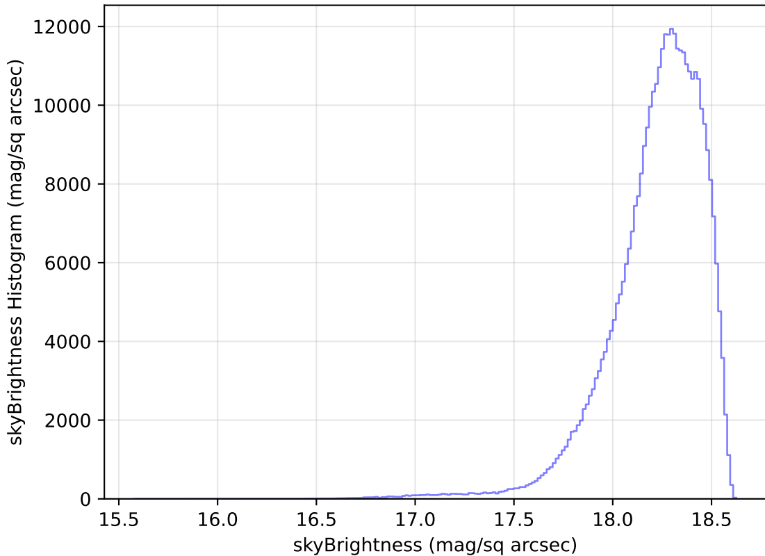
too_elab_r64_d2_giz_v3.4_10yrs All sky y band: skyBrightness Histogram
