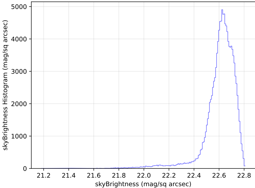
too_elab_r64_d2_giz_v3.4_10yrs All sky u band: skyBrightness Histogram
