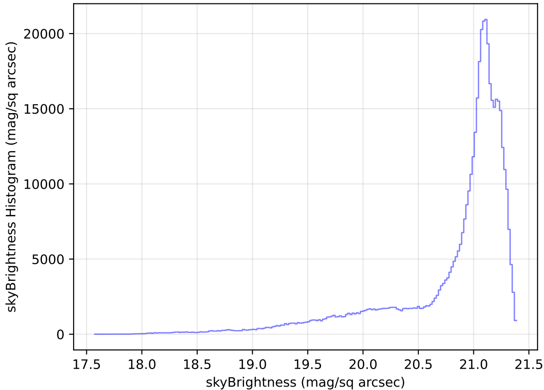
too_elab_r64_d2_giz_v3.4_10yrs All sky r band: skyBrightness Histogram
