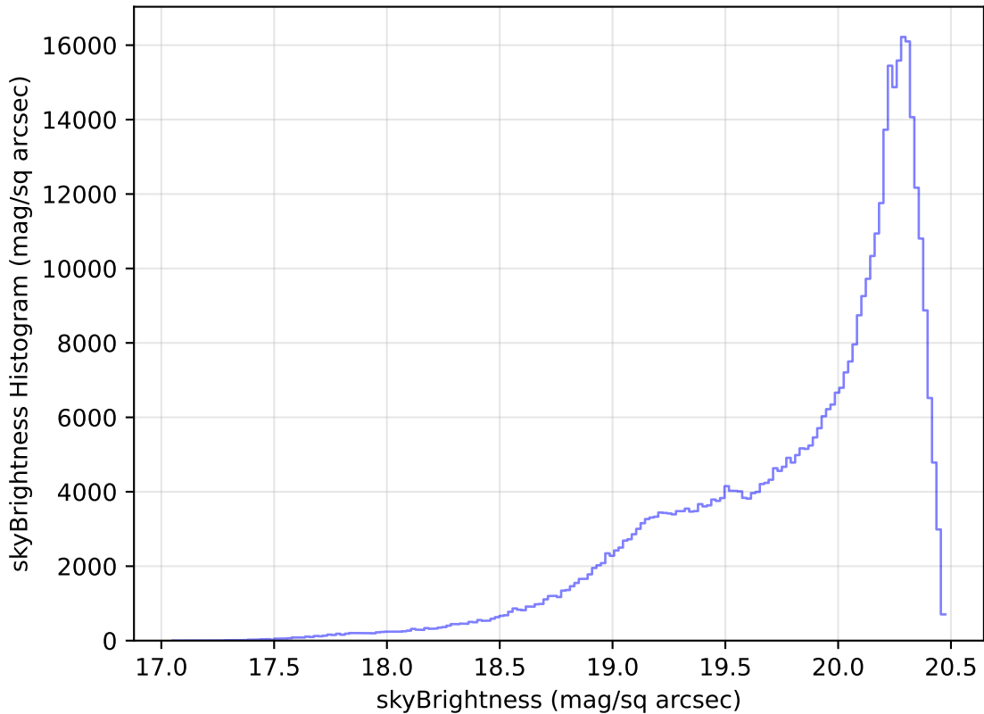
too_elab_r64_d2_giz_v3.4_10yrs All sky i band: skyBrightness Histogram
