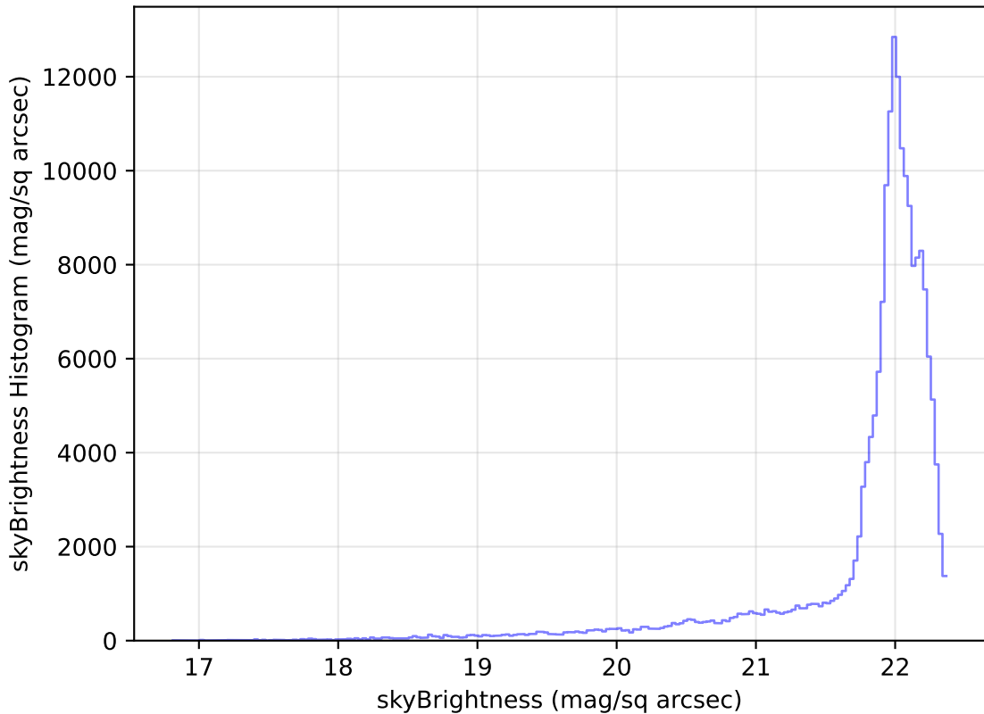
too_elab_r64_d2_giz_v3.4_10yrs All sky g band: skyBrightness Histogram
