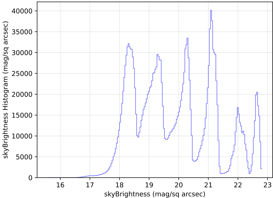
too_elab_r64_d2_giz_v3.4_10yrs All sky all bands: skyBrightness Histogram
