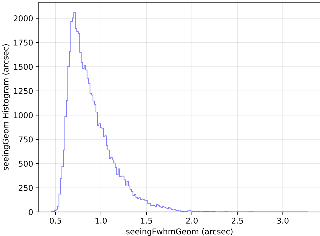
too_elab_r64_d2_giz_v3.4_10yrs Yr 1 r band: seeingGeom Histogram
