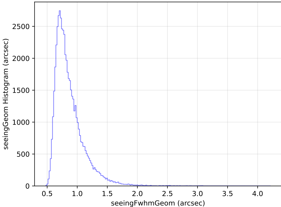
too_elab_r64_d2_giz_v3.4_10yrs Yr 1 i band: seeingGeom Histogram
