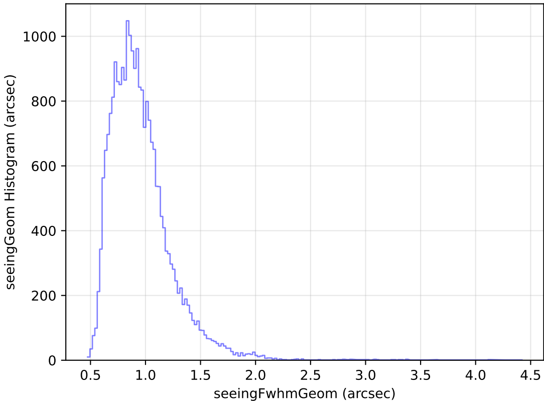
too_elab_r64_d2_giz_v3.4_10yrs Yr 1 g band: seeingGeom Histogram
