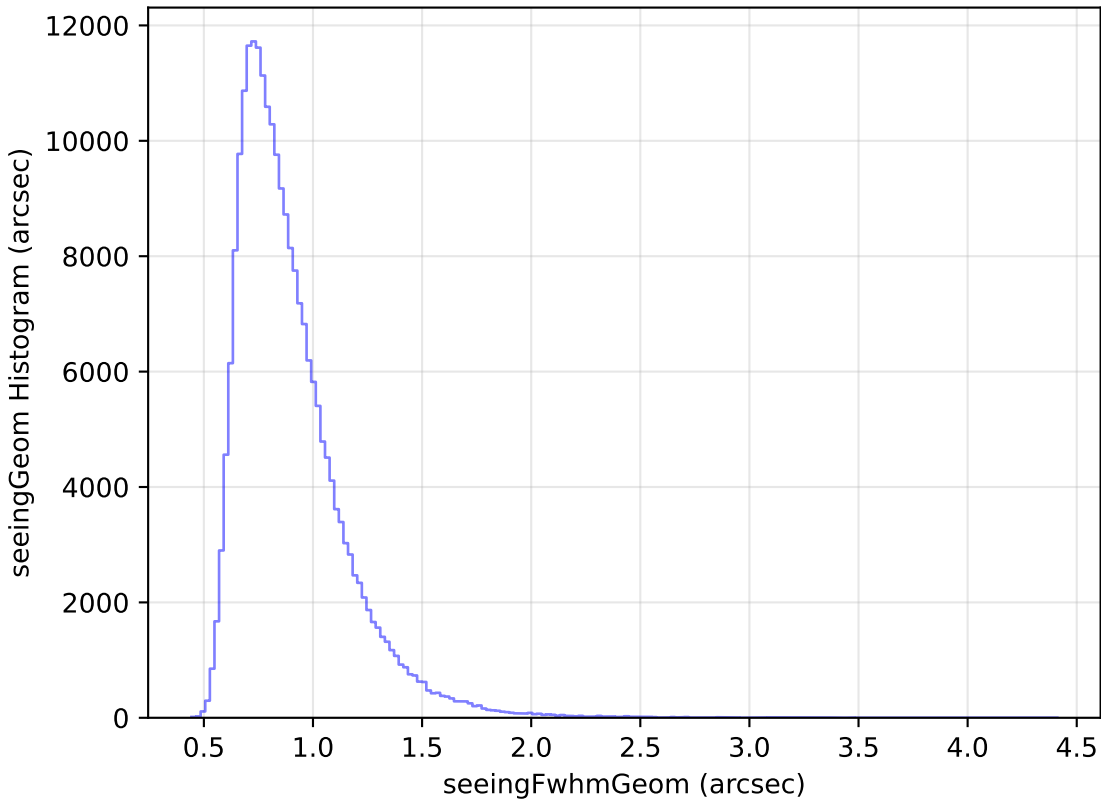
too_elab_r64_d2_giz_v3.4_10yrs Yr 1 all bands: seeingGeom Histogram
