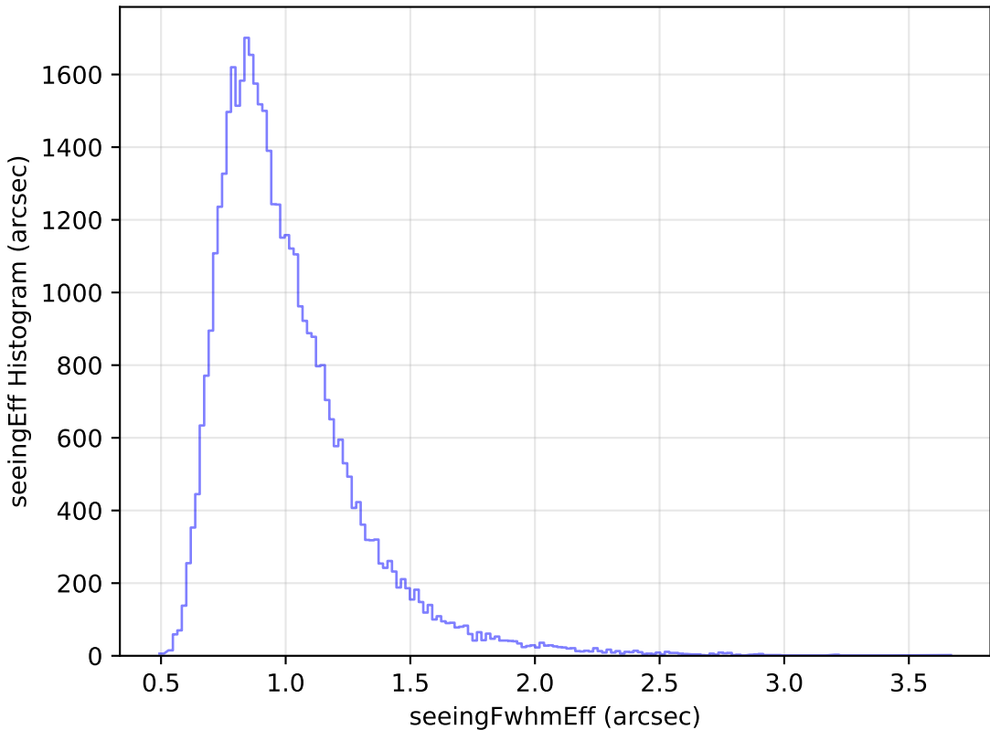
too_elab_r64_d2_giz_v3.4_10yrs Yr 1 z band: seeingEff Histogram
