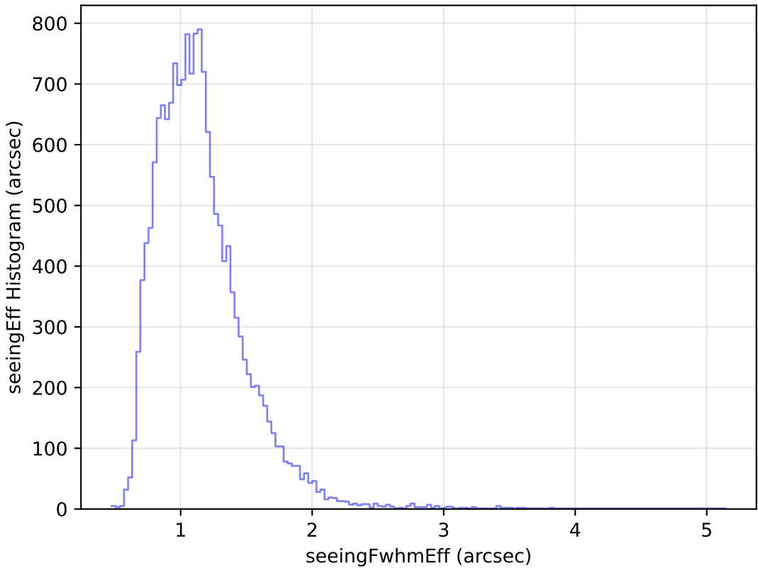
too_elab_r64_d2_giz_v3.4_10yrs Yr 1 u band: seeingEff Histogram
