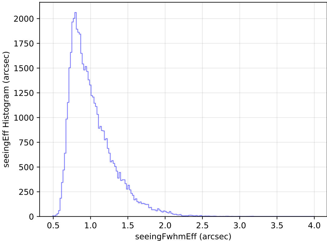
too_elab_r64_d2_giz_v3.4_10yrs Yr 1 r band: seeingEff Histogram
