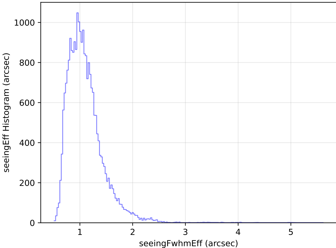
too_elab_r64_d2_giz_v3.4_10yrs Yr 1 g band: seeingEff Histogram
