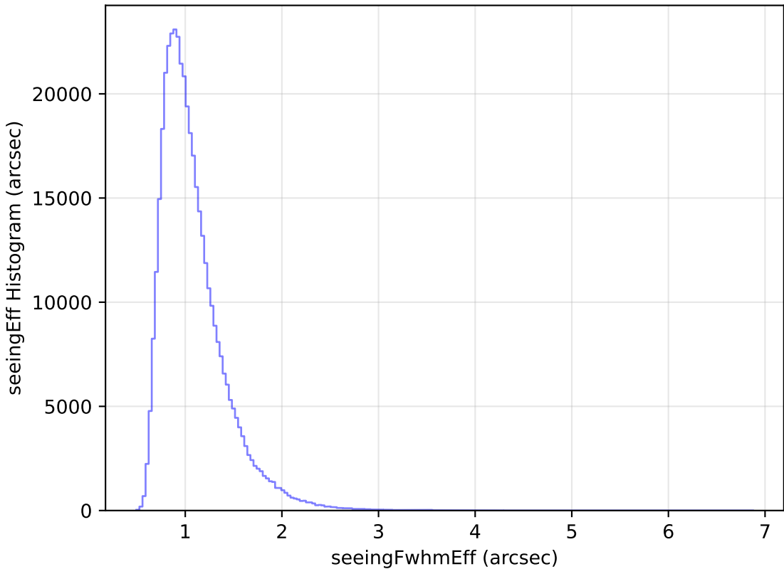
too_elab_r64_d2_giz_v3.4_10yrs WFD z band: seeingEff Histogram
