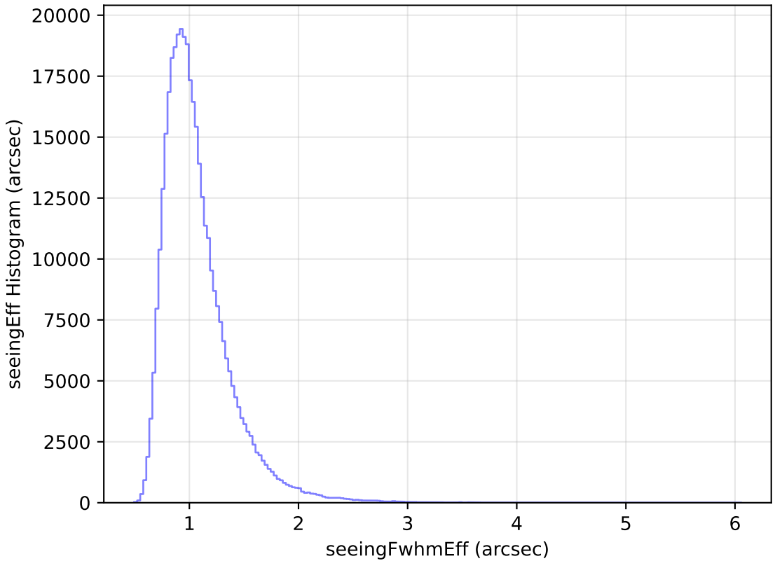
too_elab_r64_d2_giz_v3.4_10yrs WFD y band: seeingEff Histogram
