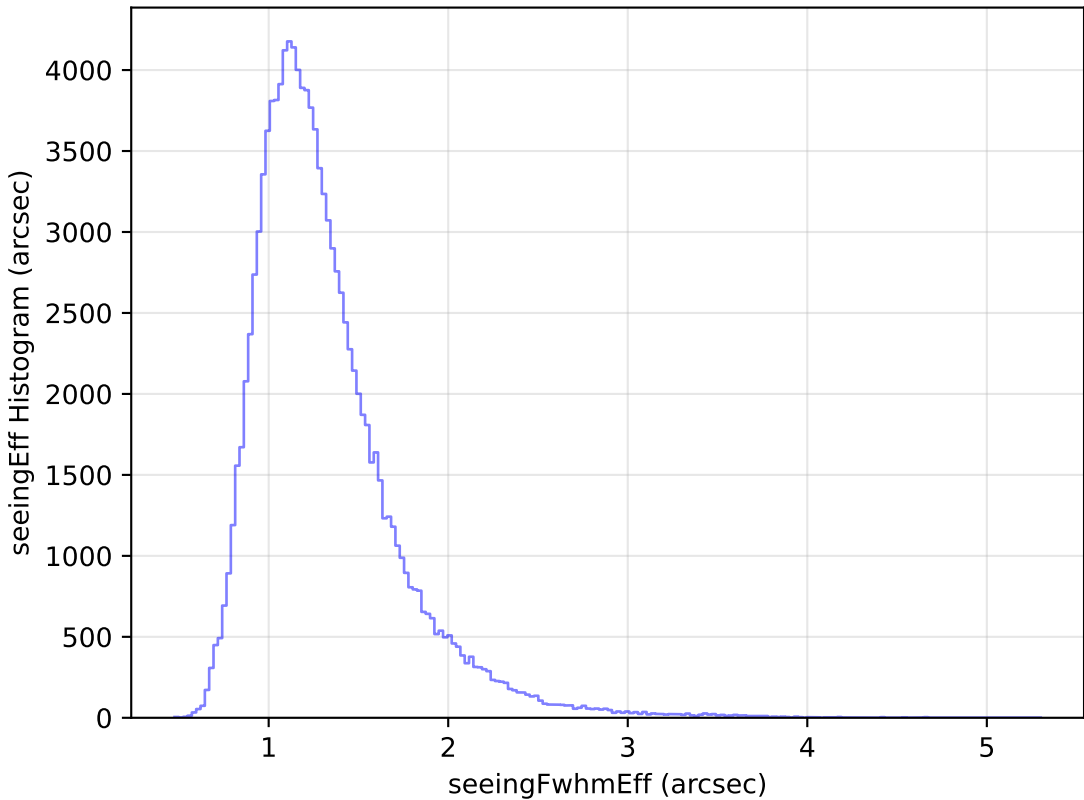
too_elab_r64_d2_giz_v3.4_10yrs WFD u band: seeingEff Histogram
