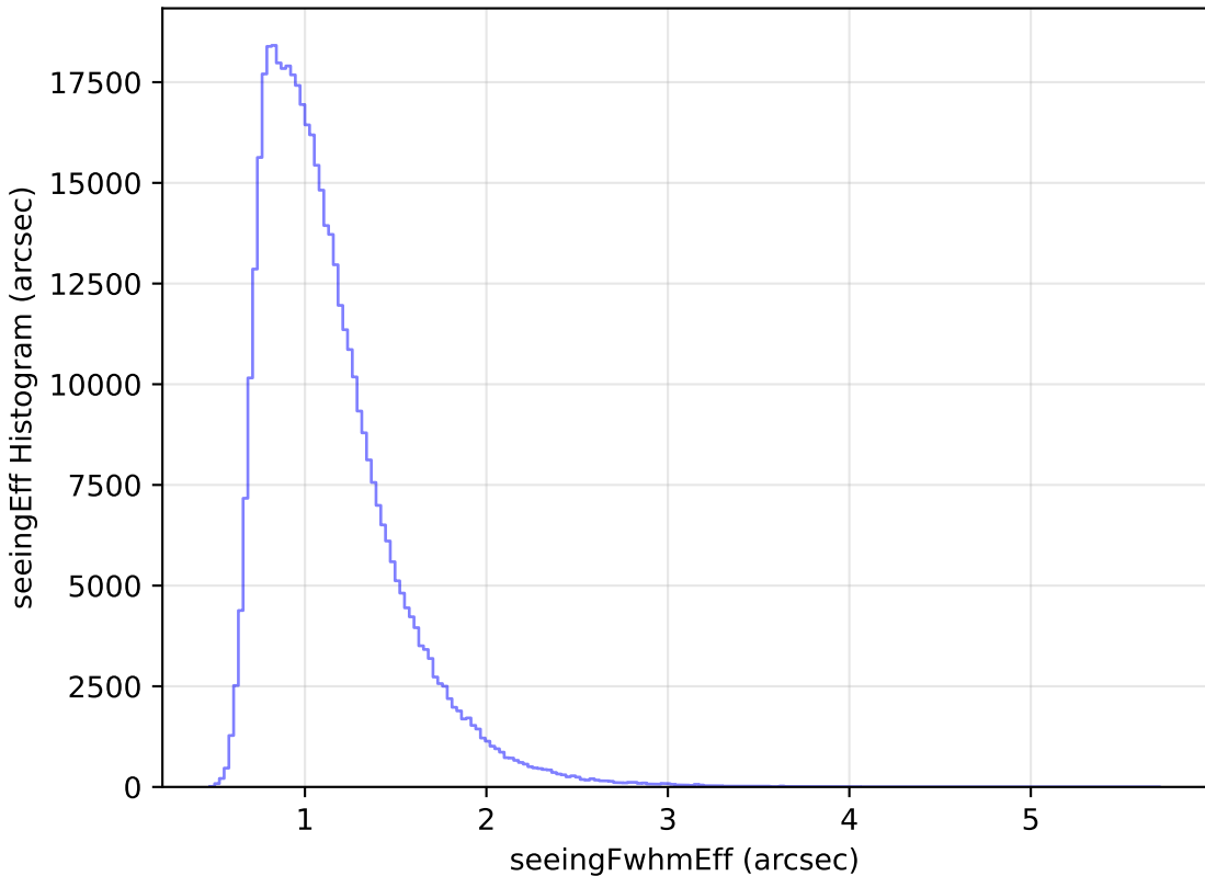
too_elab_r64_d2_giz_v3.4_10yrs WFD r band: seeingEff Histogram
