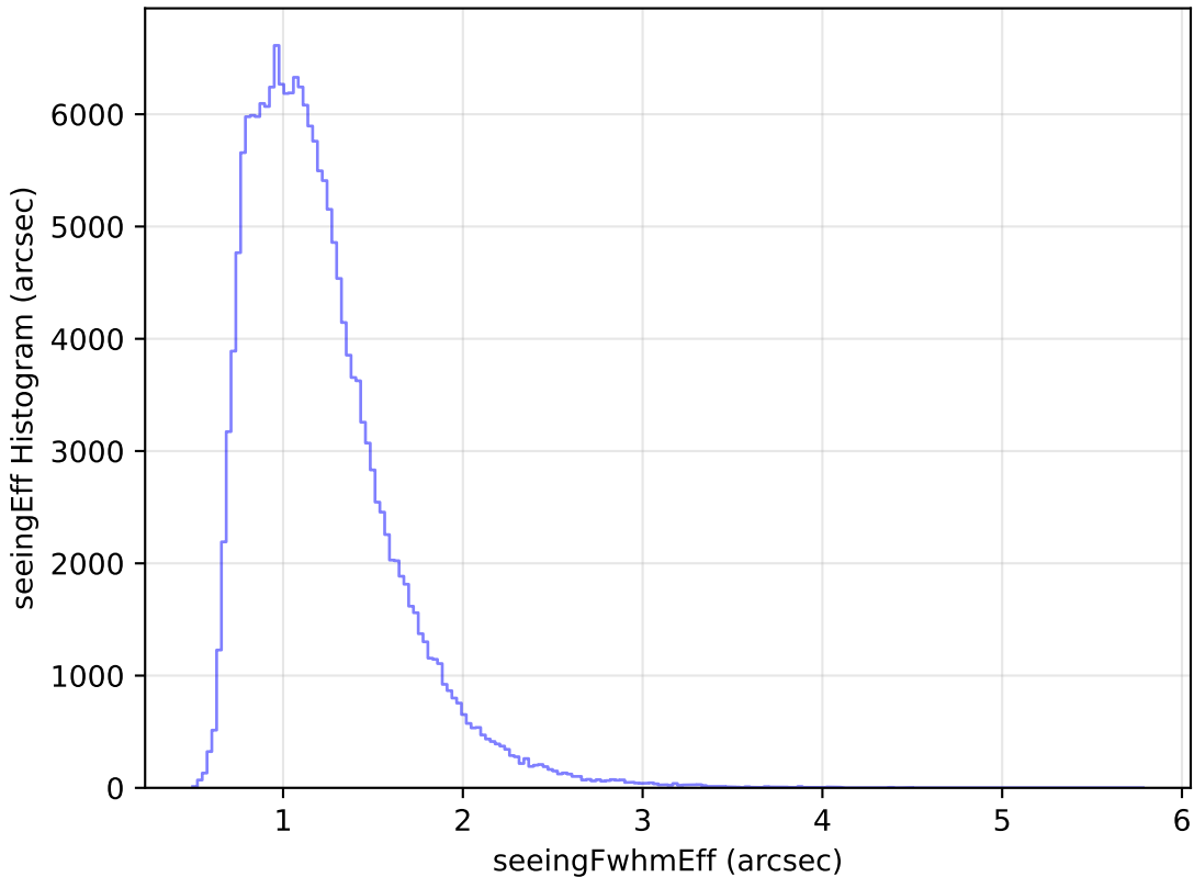
too_elab_r64_d2_giz_v3.4_10yrs WFD g band: seeingEff Histogram
