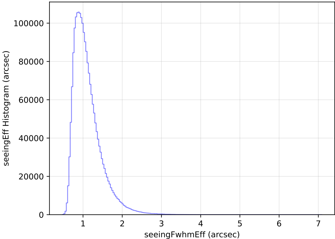
too_elab_r64_d2_giz_v3.4_10yrs WFD all bands: seeingEff Histogram
