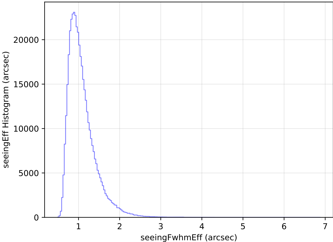
too_elab_r64_d2_giz_v3.4_10yrs All sky z band: seeingEff Histogram
