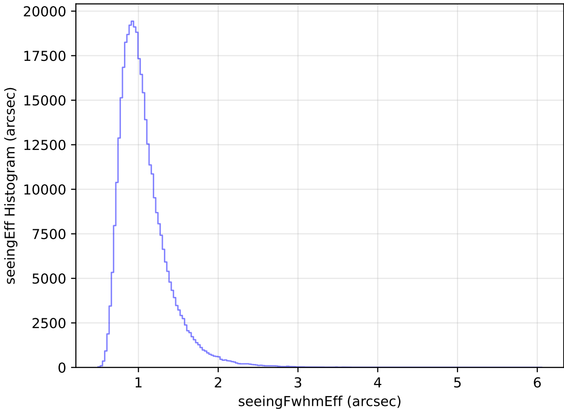
too_elab_r64_d2_giz_v3.4_10yrs All sky y band: seeingEff Histogram
