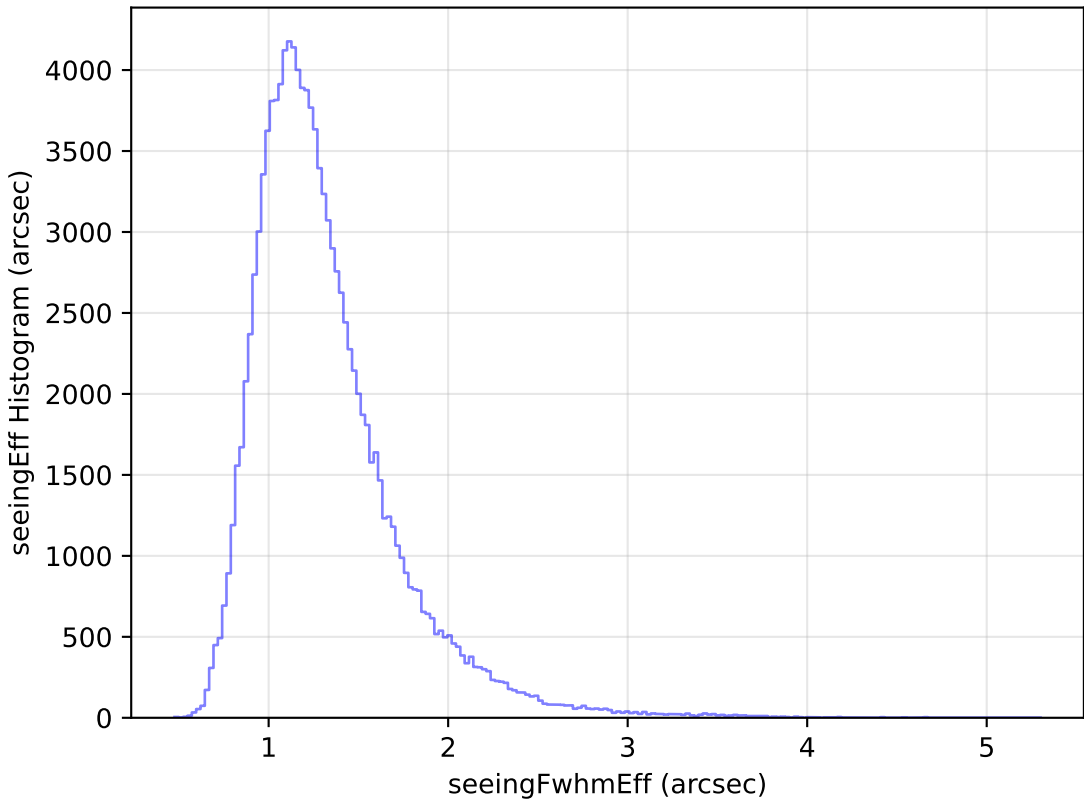
too_elab_r64_d2_giz_v3.4_10yrs All sky u band: seeingEff Histogram
