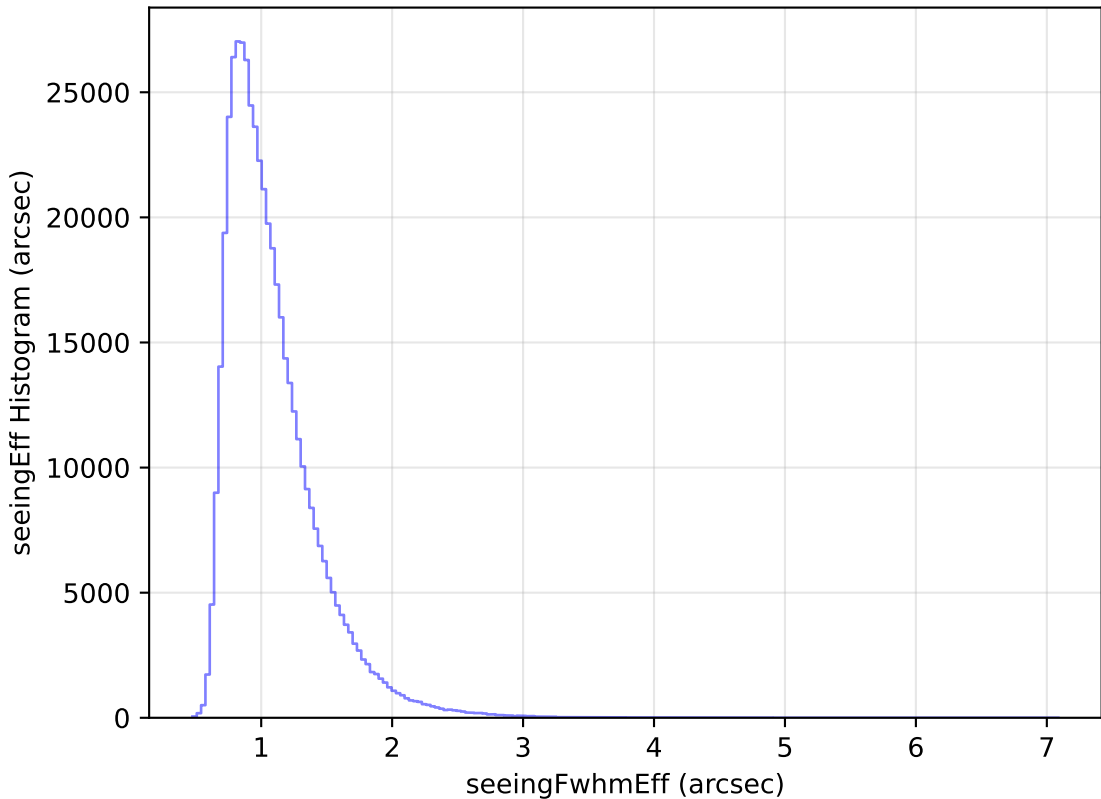
too_elab_r64_d2_giz_v3.4_10yrs All sky i band: seeingEff Histogram
