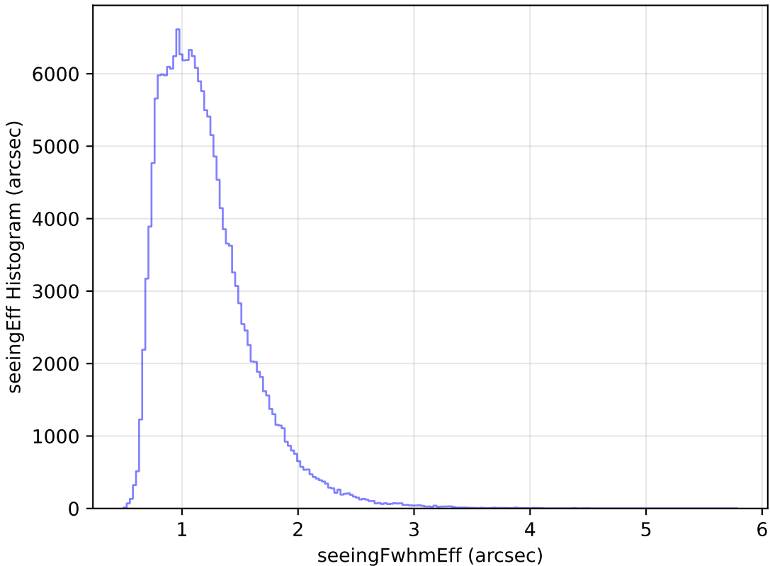
too_elab_r64_d2_giz_v3.4_10yrs All sky g band: seeingEff Histogram
