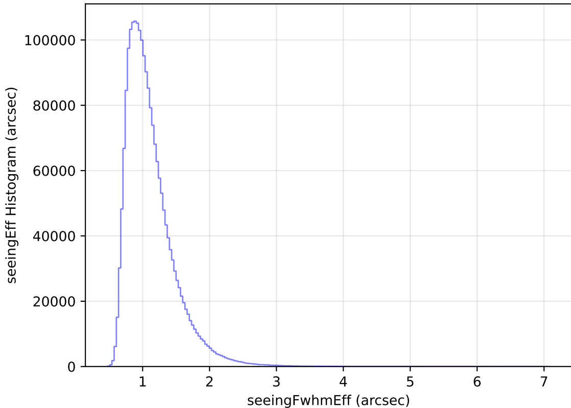
too_elab_r64_d2_giz_v3.4_10yrs All sky all bands: seeingEff Histogram
