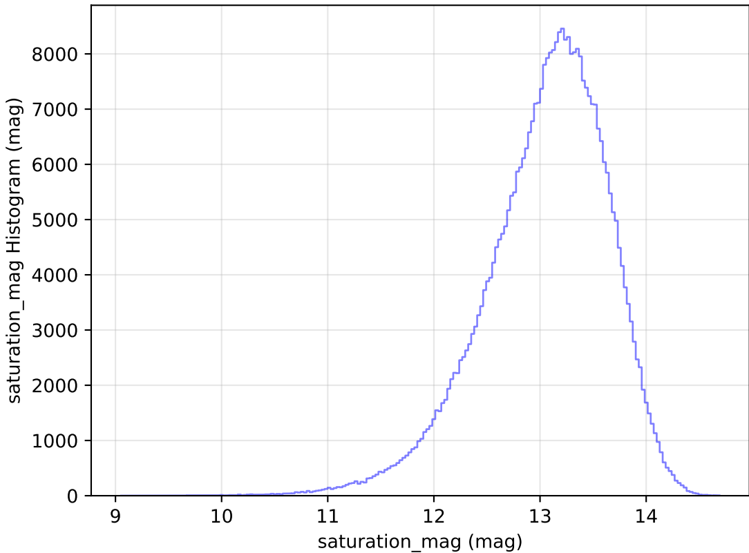
too_elab_r64_d2_giz_v3.4_10yrs WFD y band: saturation_mag Histogram
