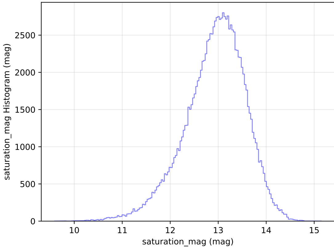
too_elab_r64_d2_giz_v3.4_10yrs WFD u band: saturation_mag Histogram
