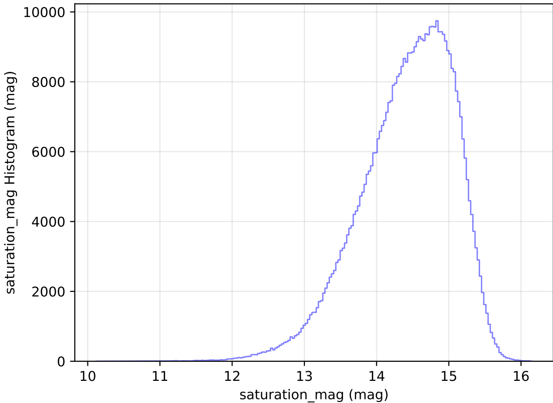
too_elab_r64_d2_giz_v3.4_10yrs WFD i band: saturation_mag Histogram
