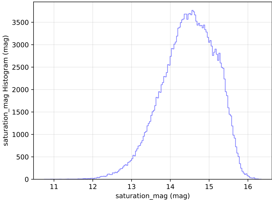
too_elab_r64_d2_giz_v3.4_10yrs WFD g band: saturation_mag Histogram
