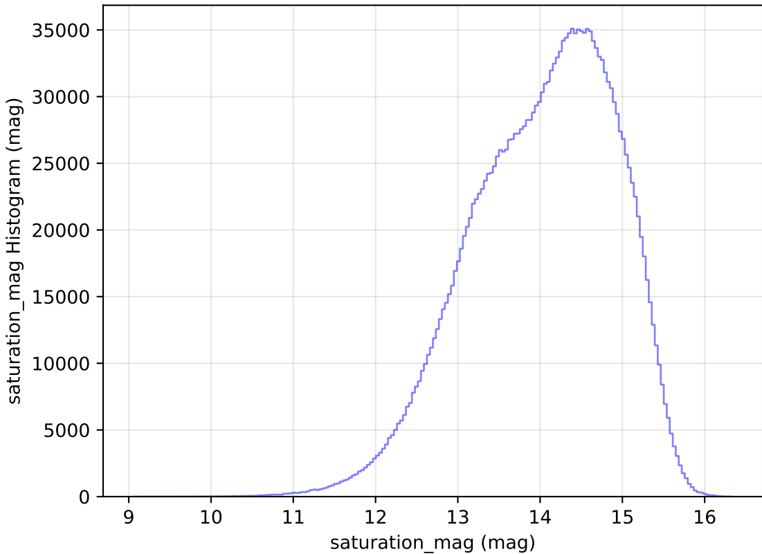
too_elab_r64_d2_giz_v3.4_10yrs WFD all bands: saturation_mag Histogram
