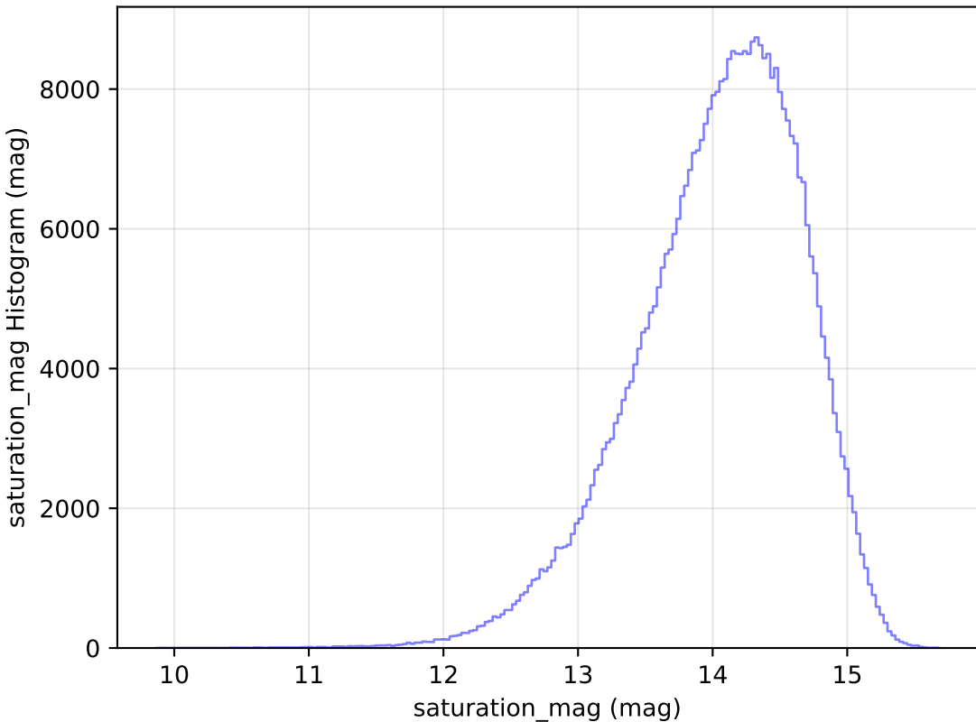
too_elab_r64_d2_giz_v3.4_10yrs All sky z band: saturation_mag Histogram
