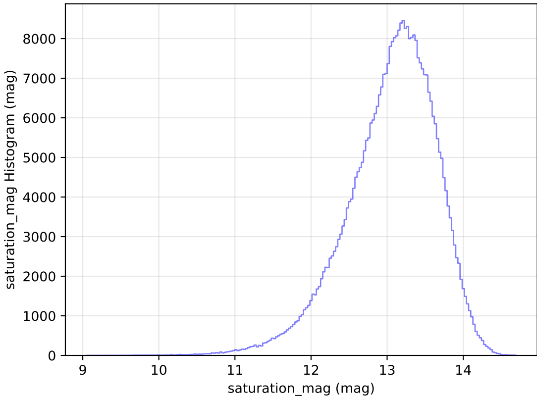
too_elab_r64_d2_giz_v3.4_10yrs All sky y band: saturation_mag Histogram
