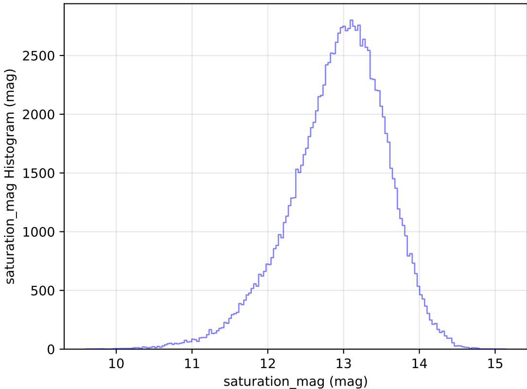
too_elab_r64_d2_giz_v3.4_10yrs All sky u band: saturation_mag Histogram
