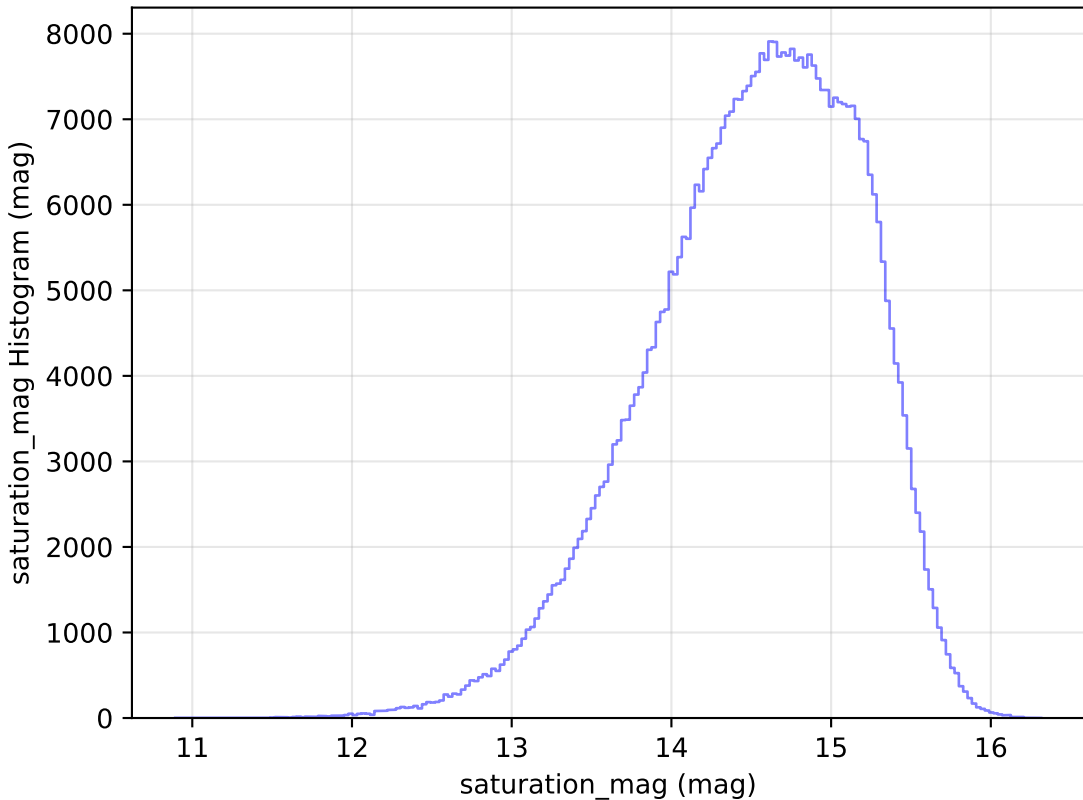
too_elab_r64_d2_giz_v3.4_10yrs All sky r band: saturation_mag Histogram
