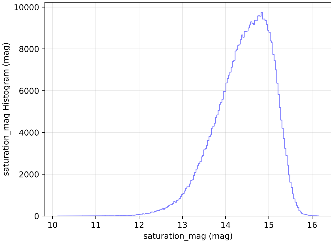
too_elab_r64_d2_giz_v3.4_10yrs All sky i band: saturation_mag Histogram
