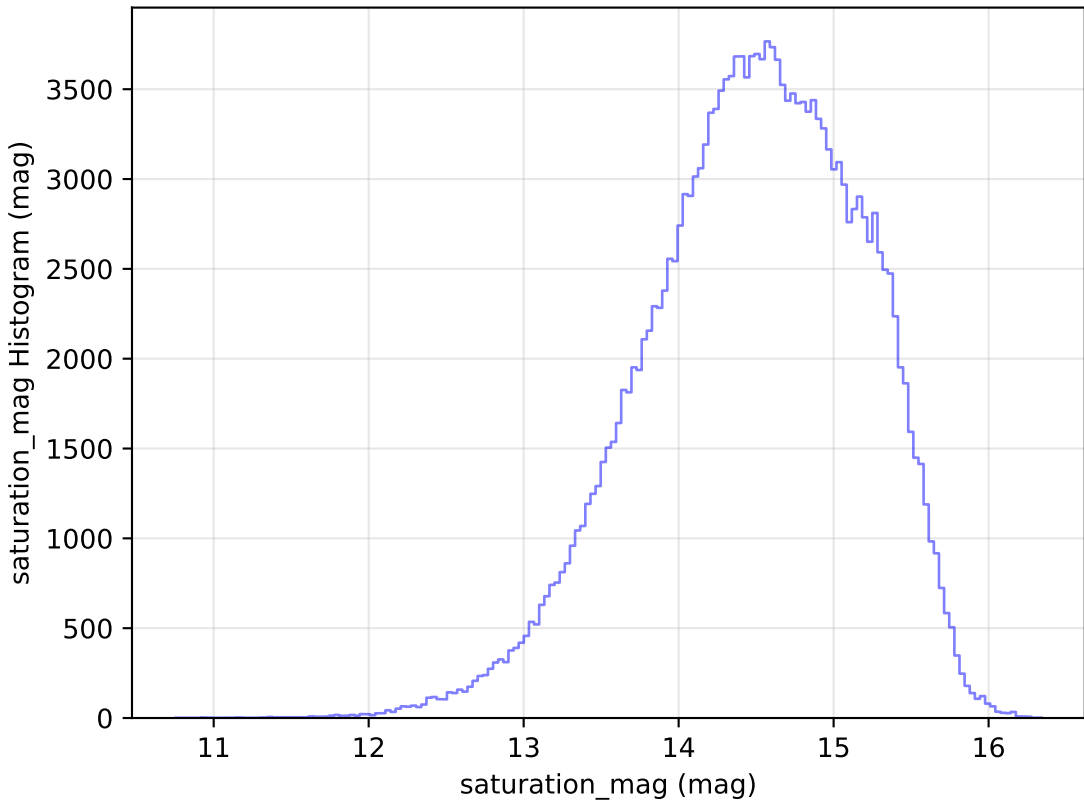
too_elab_r64_d2_giz_v3.4_10yrs All sky g band: saturation_mag Histogram
