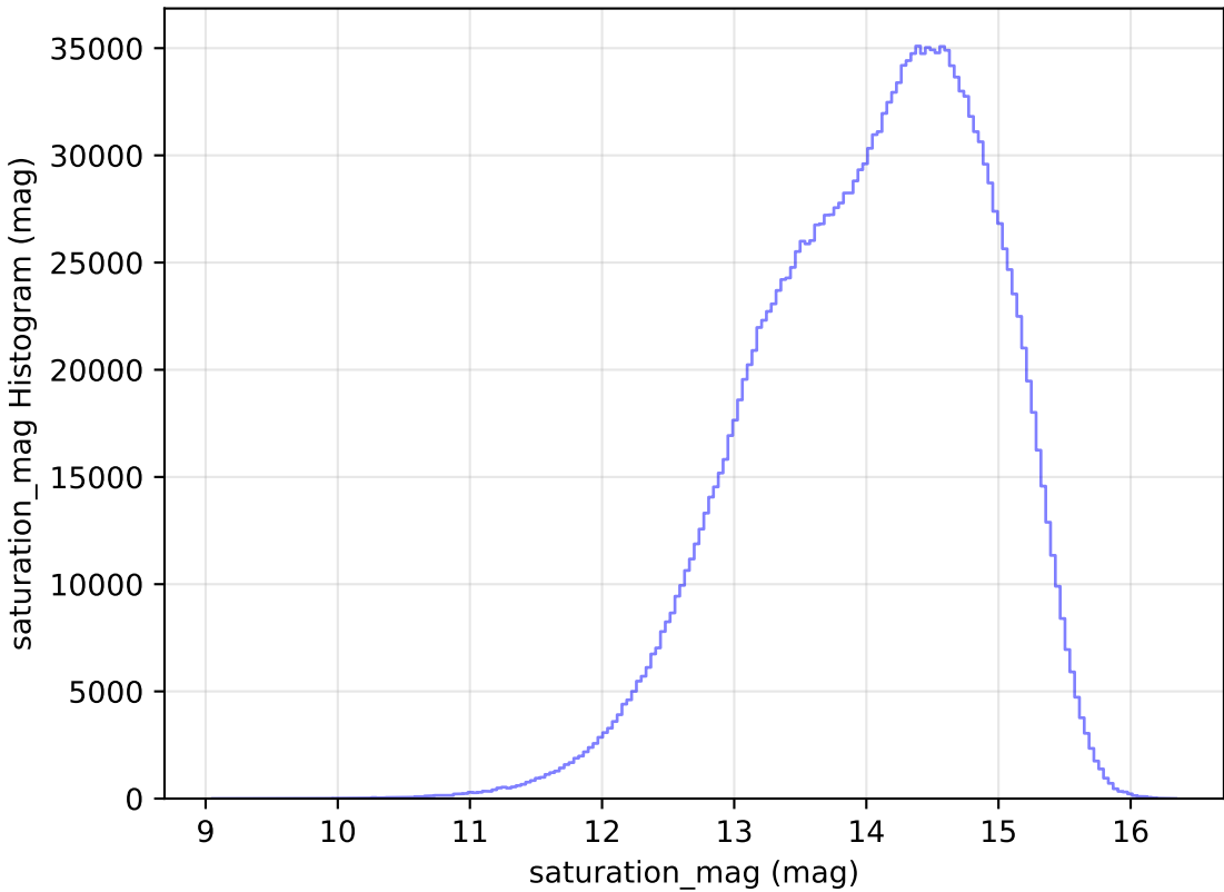
too_elab_r64_d2_giz_v3.4_10yrs All sky all bands: saturation_mag Histogram
