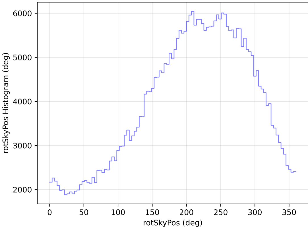
too_elab_r64_d2_giz_v3.4_10yrs WFD y band: rotSkyPos Histogram
