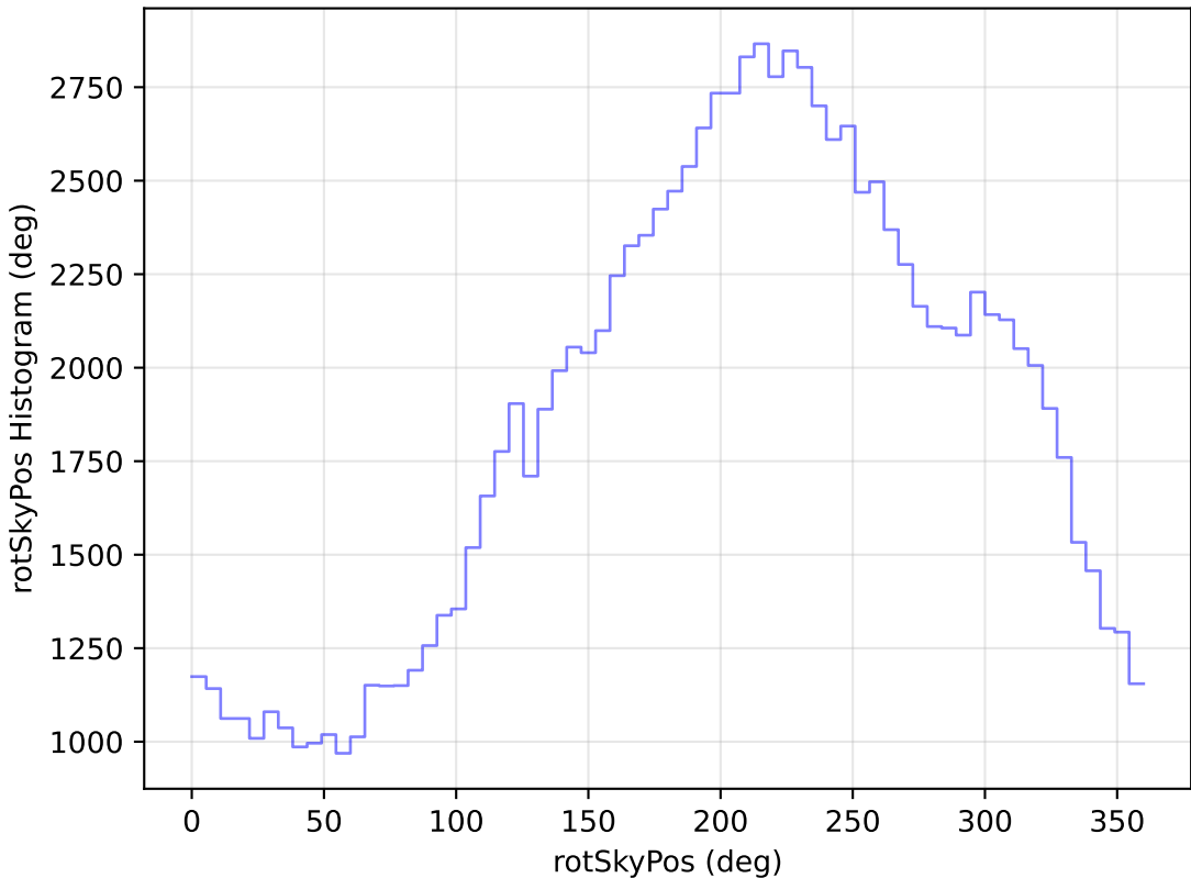
too_elab_r64_d2_giz_v3.4_10yrs WFD u band: rotSkyPos Histogram
