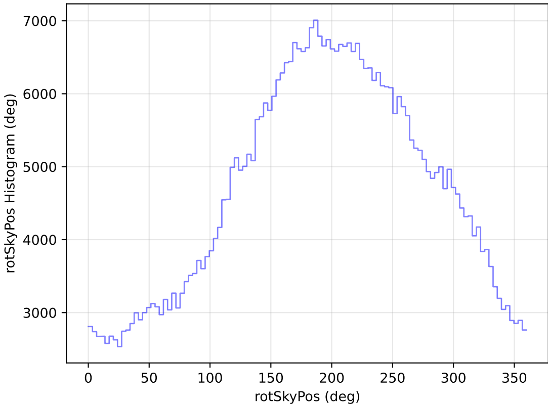
too_elab_r64_d2_giz_v3.4_10yrs WFD r band: rotSkyPos Histogram
