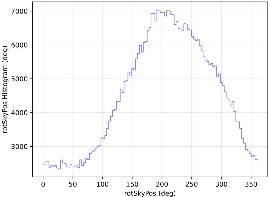
too_elab_r64_d2_giz_v3.4_10yrs WFD i band: rotSkyPos Histogram
