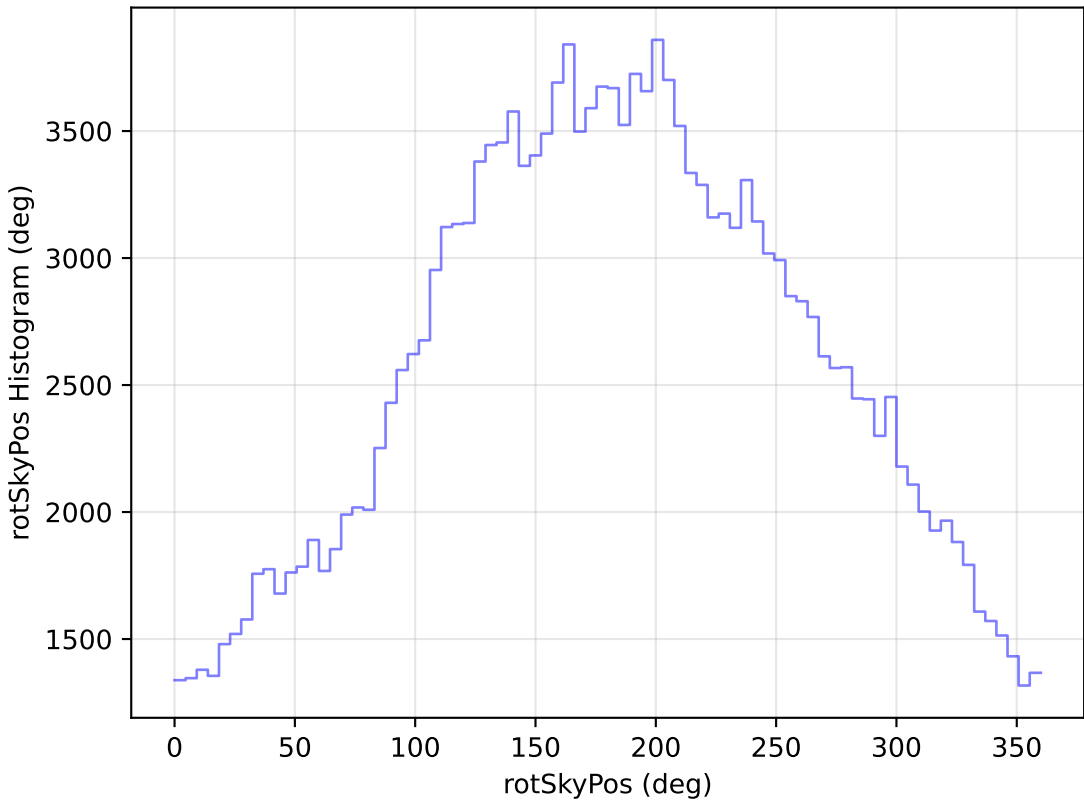
too_elab_r64_d2_giz_v3.4_10yrs WFD g band: rotSkyPos Histogram
