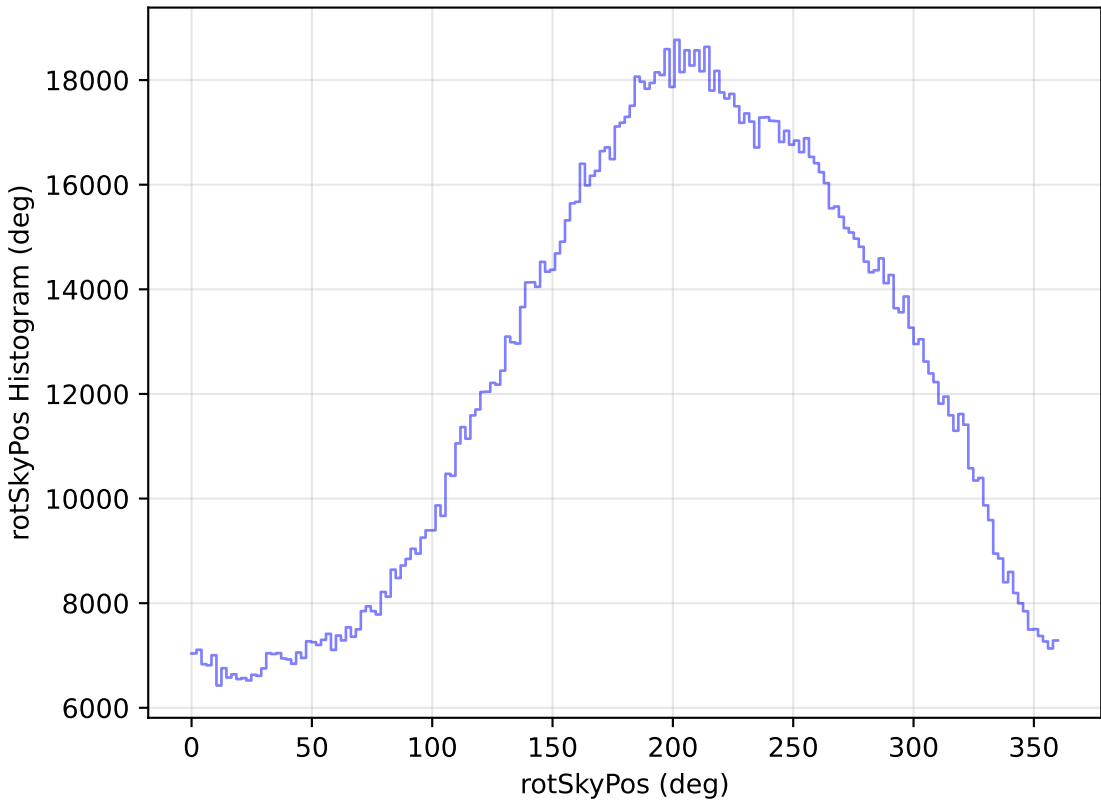
too_elab_r64_d2_giz_v3.4_10yrs WFD all bands: rotSkyPos Histogram
