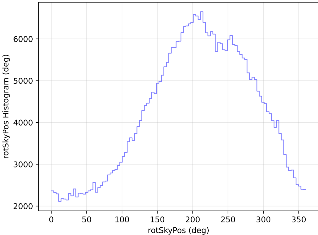
too_elab_r64_d2_giz_v3.4_10yrs All sky z band: rotSkyPos Histogram
